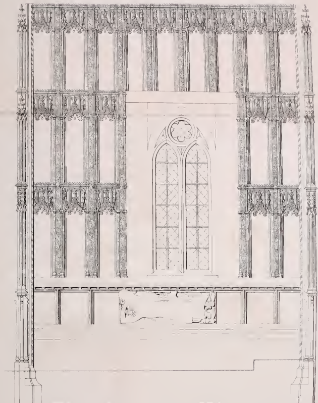
ELEVATION OF REREDOS AT EAST END OF TANNERS CHAPEL ST CUTHBERTS CHURCH, WELLS, SOMERSET
