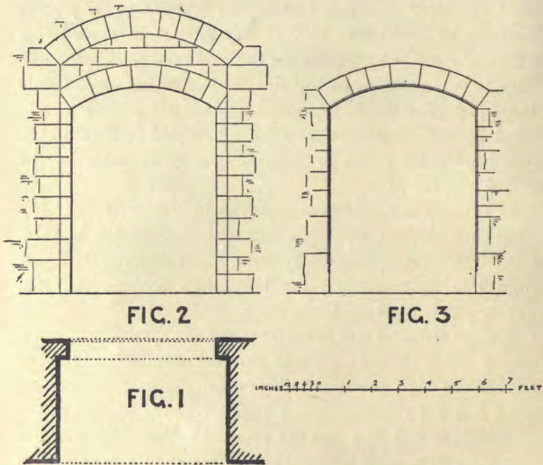
Figs. 1, 2, and 3. Plan, inner and outer elevations of arched entrance to Norman Keep, which is probably one of the oldest features in the masonry of the Castle.
