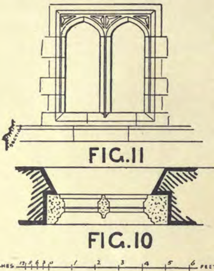
Figs. 10 and 11. Plan and elevation of window, corresponding with adjacent older windows, inserted in north wall of Castle House in place of modern cupboard.
